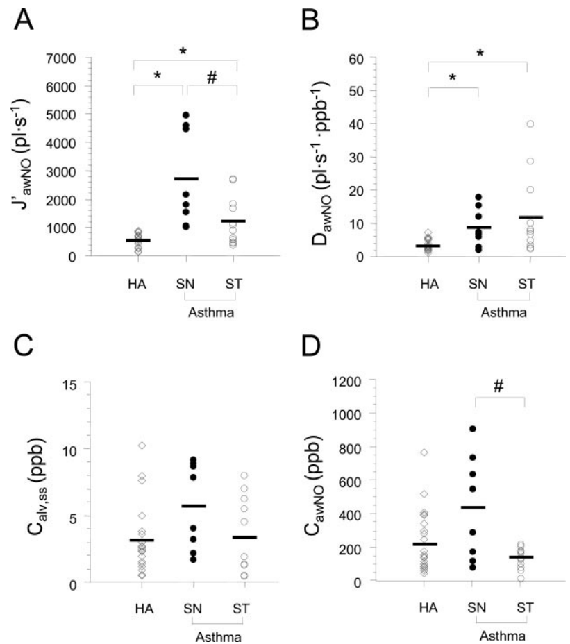
Fig. 5. Individual and population mean (solid bar) values of 4 flow-independent parameters (A: J'_{awNO} ; B: D_{awNO} ; C: C_{alv,ss} ; D: C_{awNO} ) for SN (●) and ST (○) asthma subjects and HA (◇). The mean \pm SD J'_{awNO} , D_{awNO} , C_{alv,ss} , and C_{awNO} for HA, SN, and ST are as follows: HA: 530 \pm 234 pl/s, 3.13 \pm 1.57 pl·s -1 ·ppb -1 , 3.08 \pm 2.39 ppb, and 220 \pm 177 ppb; SN: 2,693 \pm 1,687 pl/s, 8.71 \pm 5.74 pl·s -1 ·ppb -1 , 5.68 \pm 3.22 ppb, and 438 \pm 312 ppb; ST: 1,196 \pm 837 pl/s, 11.8 \pm 11.7 pl·s -1 ·ppb -1 , 3.30 \pm 2.74 ppb, and 143 \pm 66 ppb, respectively. Statistically different from *HA and #SN subjects with asthma: P < 0.05 .
