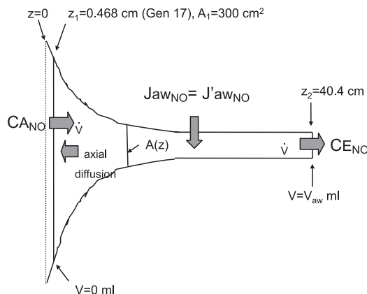
Fig. 1. Schematic of the trumpet model. Alveolar air with nitric oxide (NO) steady-state alveolar concentration ( C_{A_{NO}} ) exits the alveolar region at position z_1 (generation 17) and is transported toward the mouth (position z_2 ) by convection at a steady volumetric flow rate ( V ). NO is added to the airstream at a rate equal to the wall flux of NO from the airway wall ( J_{awNO} ; pl/s). Because the flow is larger than 100 ml/s, J_{awNO} can be considered constant and equal to the maximum airway flux J'_{awNO} (9). Thus the concentration increases with z -position and the concentration at the mouth (the exhaled concentration, C_{ENO} ) is described by Eq. 2. Axial diffusion of NO is described by Fick's 1st law of diffusion and transports NO from high to low concentration; thus NO is simultaneously transported by diffusion in the axial direction back toward the alveolar region. Airway volume is defined as the volume between positions z_1 and z_2 and is estimated in ml as the sum of the subjects age in years plus ideal body weight in pounds (5, 33). The cross-sectional area of the trumpet decreases with increasing z -position and is determined by the relationship in Eq. 1 by mapping the airway dimensions to that of the Weibel symmetric bifurcating airway tree (37).
